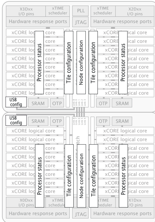
Figure 35: Registers
